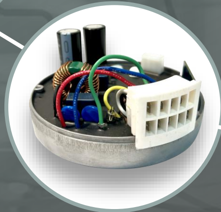
HVAC blower motor sub assembly
